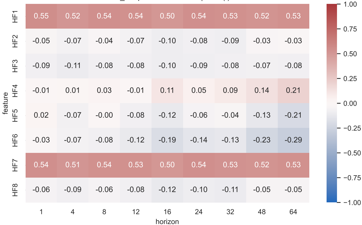
CS2_37: partial correlation | SOH(t)
