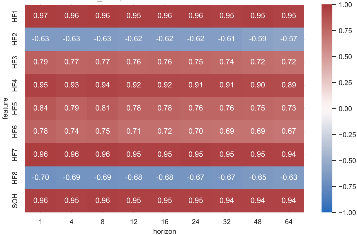
CS2_38: Spearman correlation with future SOH
