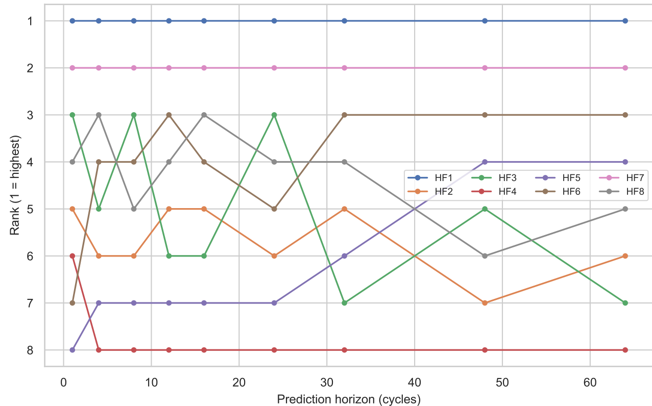
CS2_38: partial-correlation rank evolution
