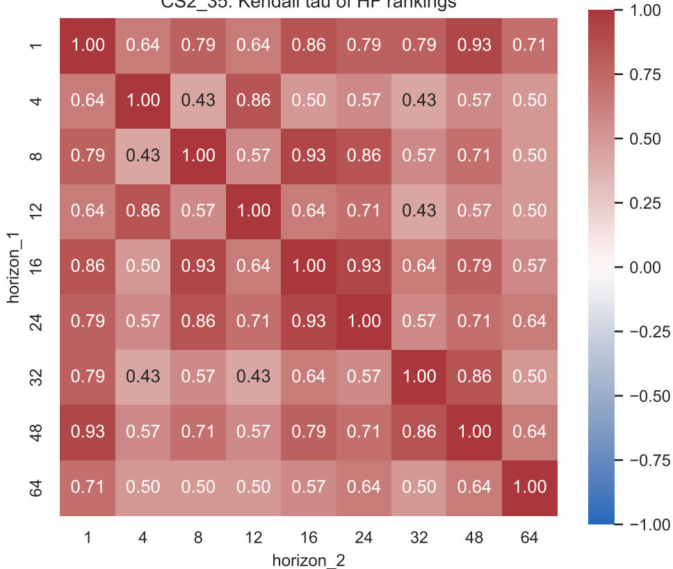
CS2_35: Kendall tau of HF rankings
