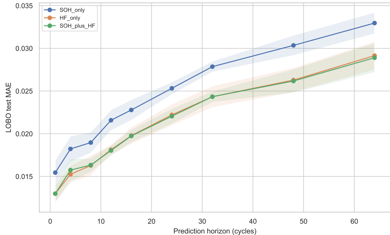
Ridge prediction probe: mean \pm SD
