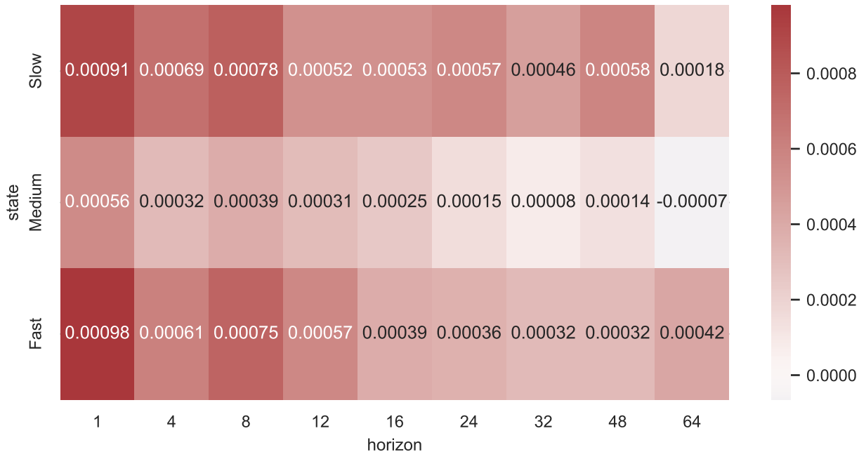
V2.5-3 Group_CC utility: state × horizon
