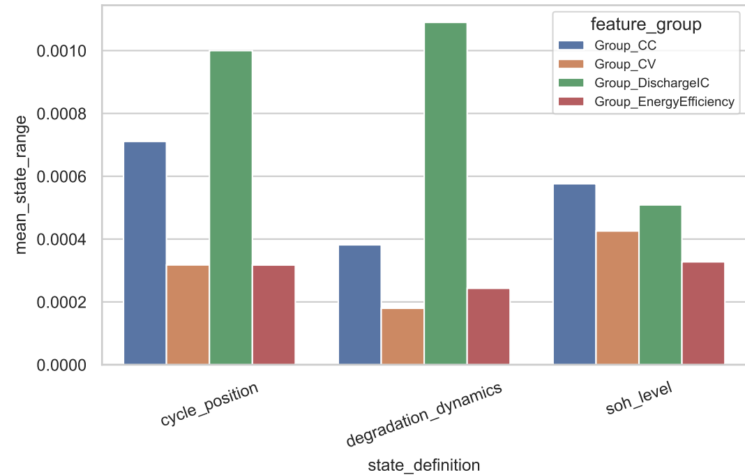
Mean utility range across states
