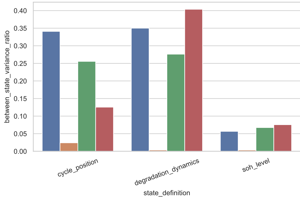
Between-state variance ratio
