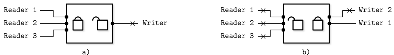
Figure 5-8. Readers-writer locks
