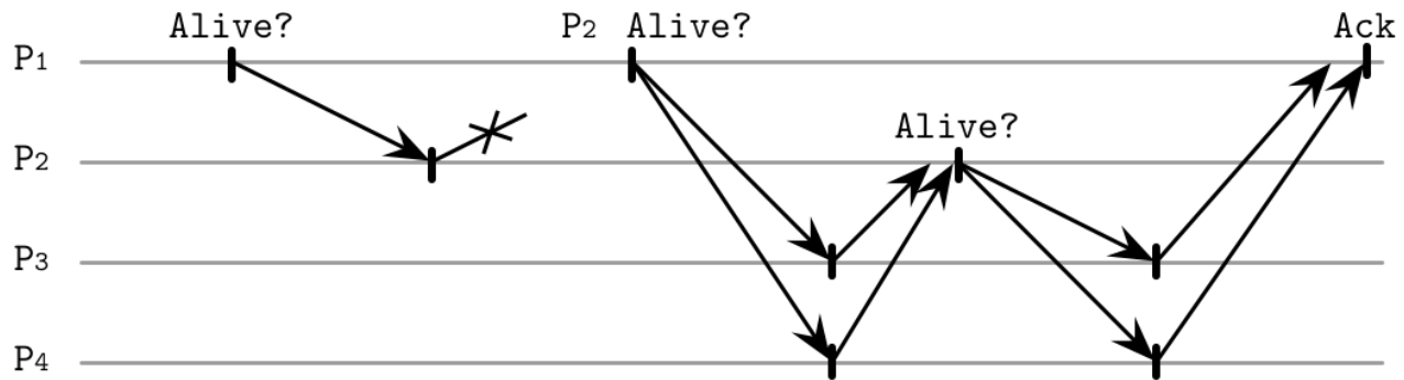
Figure 9-3. “Outsourcing” heartbeats
