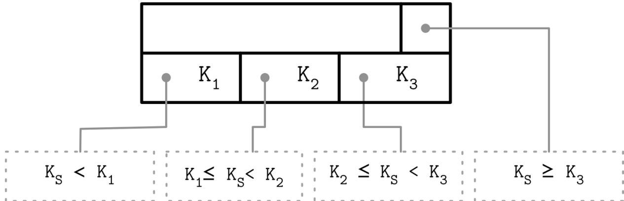
Figure 4-2. Rightmost pointer
