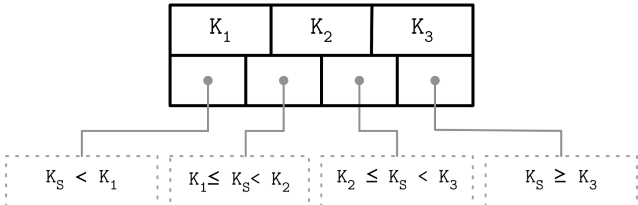
Figure 2-10. How separator keys split a tree into subtrees Some B-Tree variants also have sibling node pointers, most often on the leaf level, to simplify range scans. These pointers help avoid going back to the parent to find the next sibling. Some implementations have pointers in both directions, forming a double-linked list on the leaf level, which makes the reverse iteration possible.
