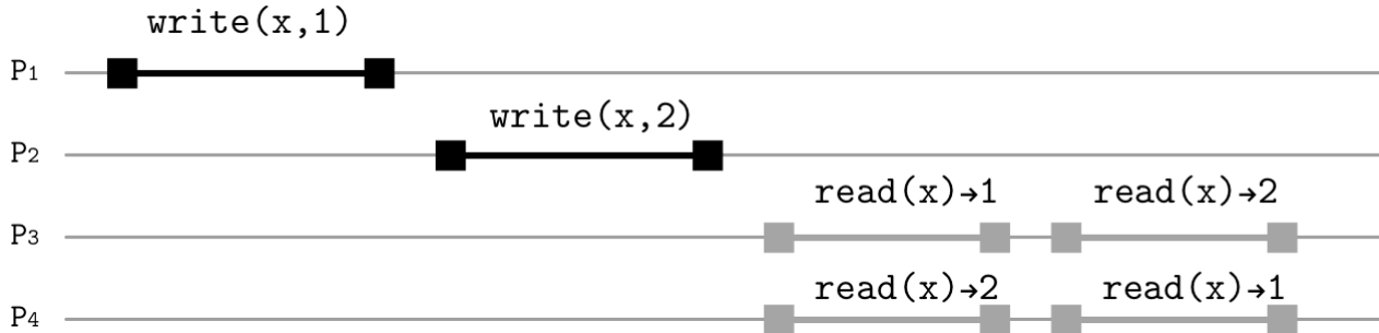
Figure 11-6. Write operations with no causal relationship
