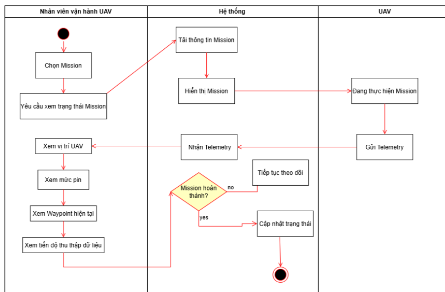
Hình 7: Activity Diagram Monitor Mission
