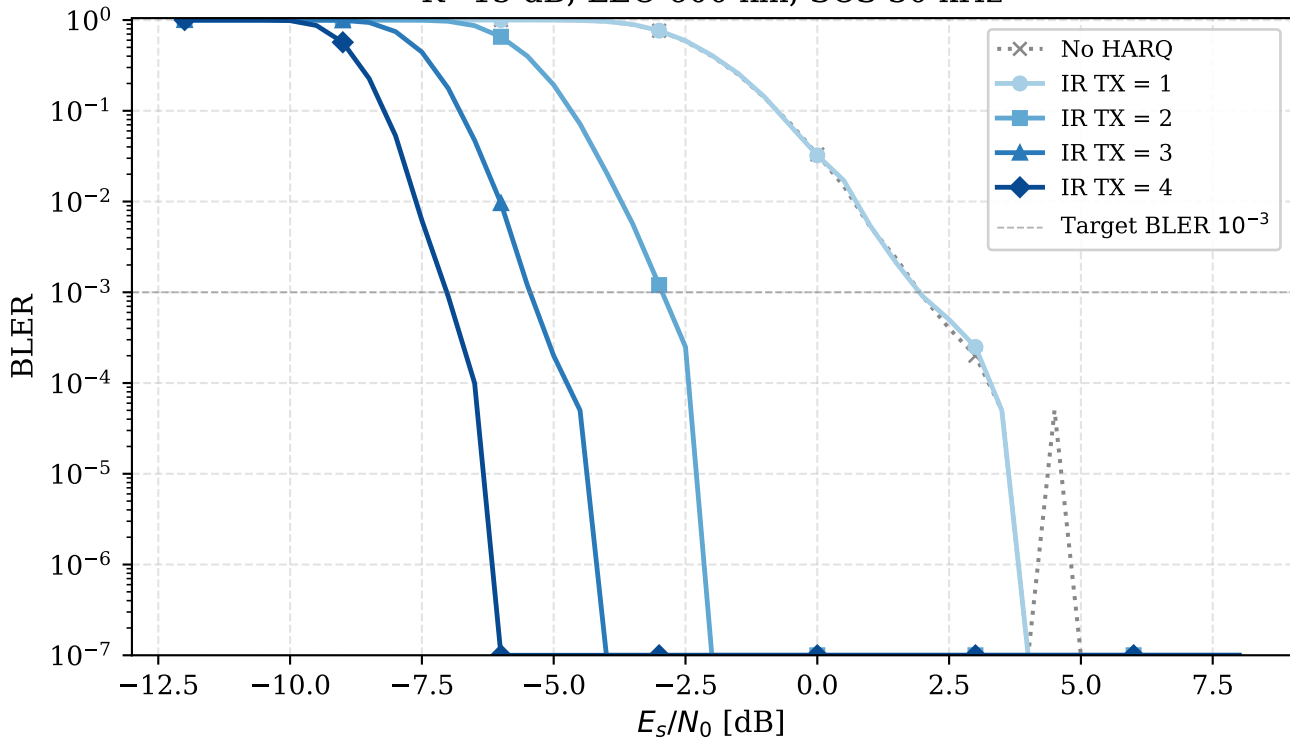
BLER vs E_s/N_0 — IR-HARQ, MCS A (QPSK r=1/2) K=15 dB, LEO 600 km, SCS 30 kHz
