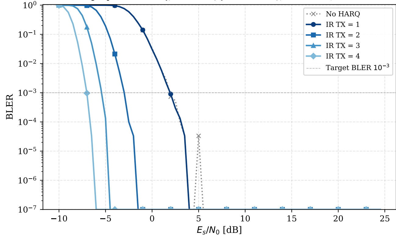
BLER vs E_s/N_0 -- IR-HARQ, MCS A (QPSK r=1/2), K=15 dB, LEO 600 km
