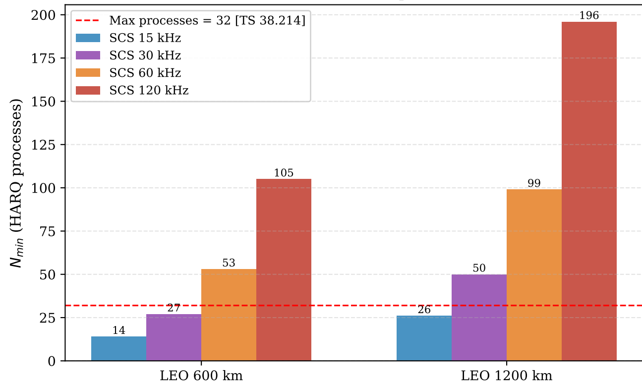
Minimum HARQ Processes Required -- LEO Orbits
