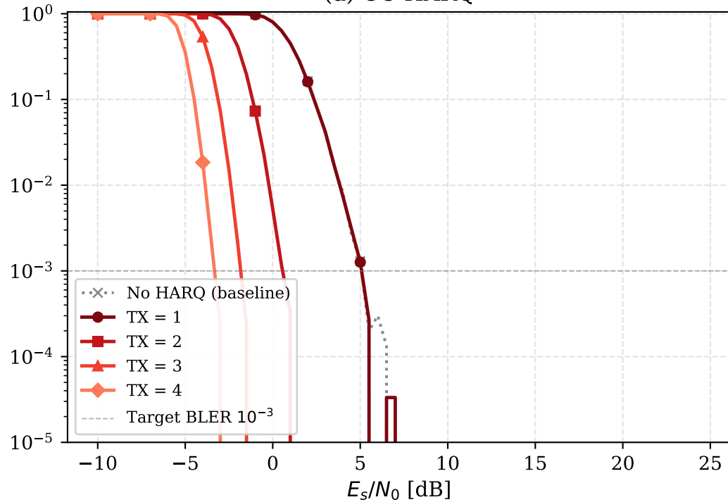
(a) CC-HARQ
