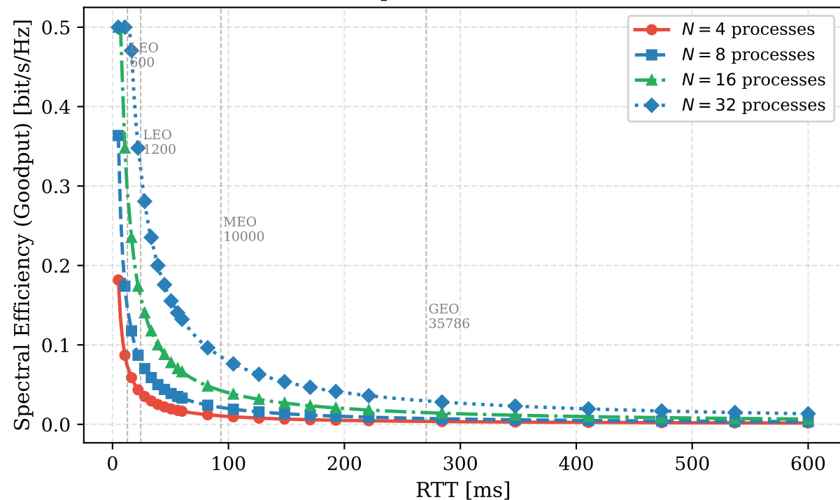
SE Goodput vs RTT — IR-HARQ
