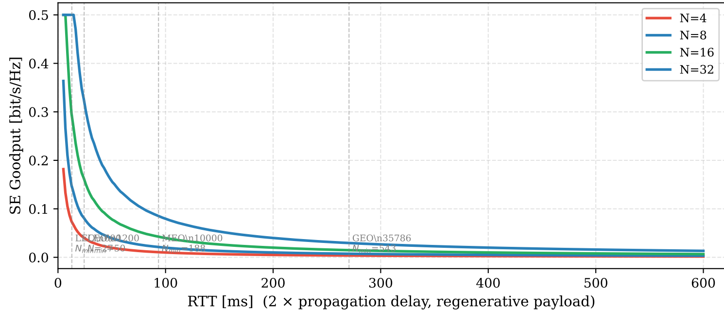
Throughput Collapse vs RTT for Different HARQ Process Counts [SCS 30 kHz, MCS A, IR-HARQ, K = 15 dB, E_s/N_0 = 5 dB]
