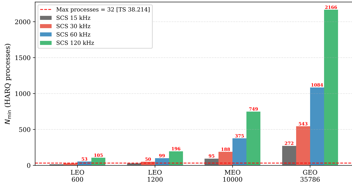
Minimum HARQ Processes Required to Avoid Pipeline Stall
