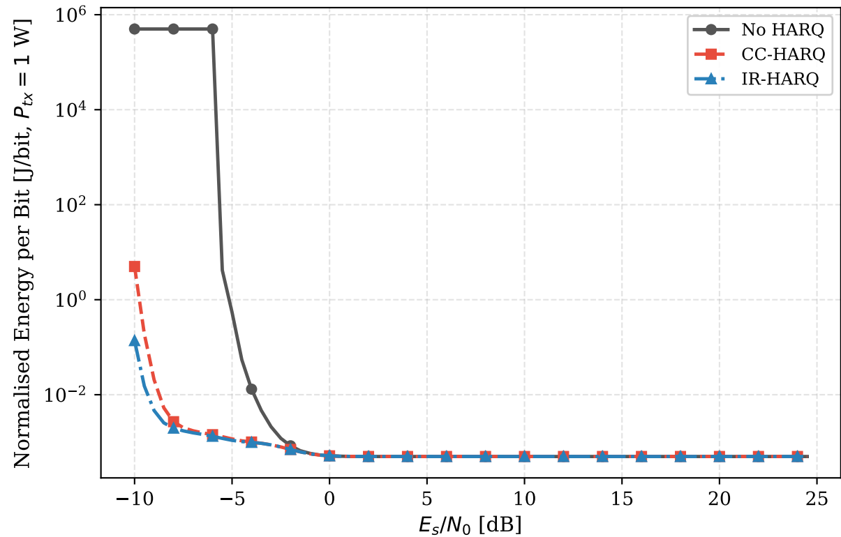
Energy Efficiency vs SNR — LEO 600 km, K = 15 dB
