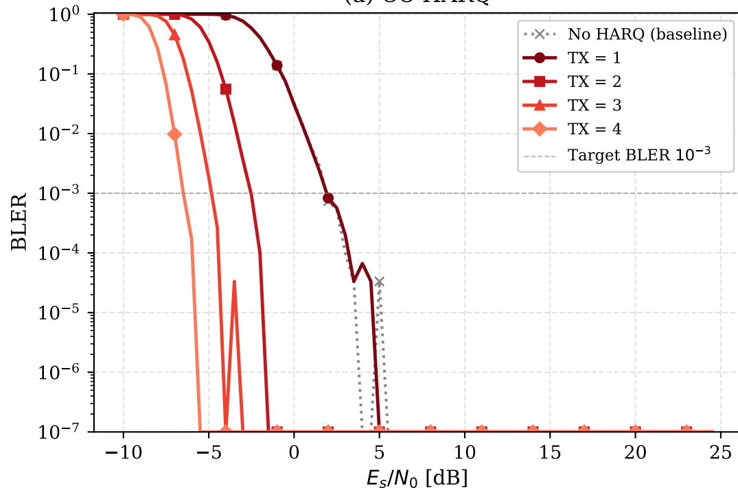
(a) CC-HARQ
