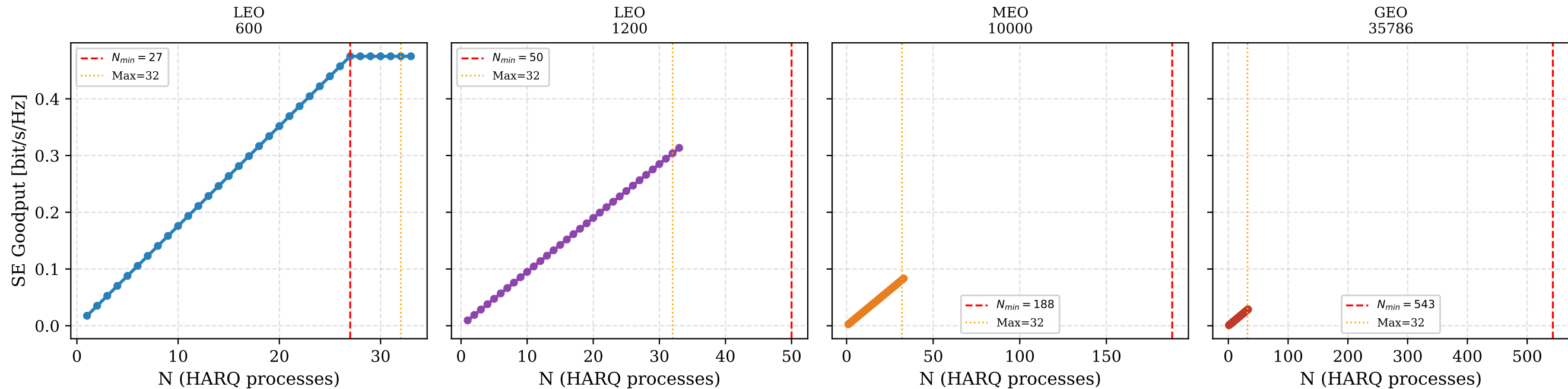
SE Goodput vs N_processes per Orbit [SCS 30 kHz, K = 15 dB]
