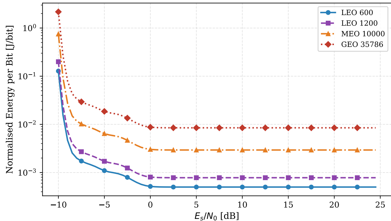
Energy Efficiency — IR-HARQ across Orbits [ N = 32 , SCS 30 kHz, MCS A, K = 15 dB]
