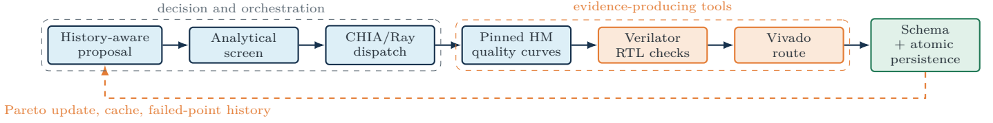
Figure 1. Complete CHIA-RDO loop. Dominated and failed points remain in history, preventing repeated proposals and turning backend failures into the next architecture decision.
