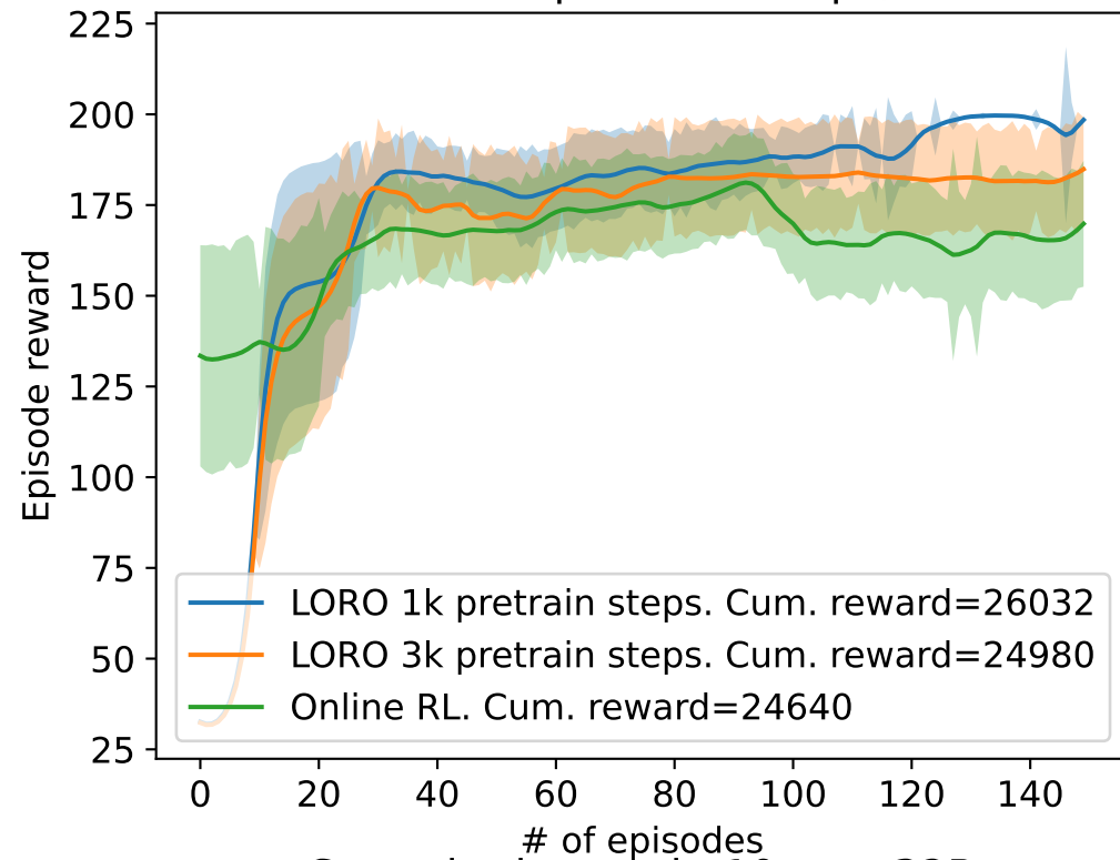
Smoothed pretrain 10 eps, 32B
