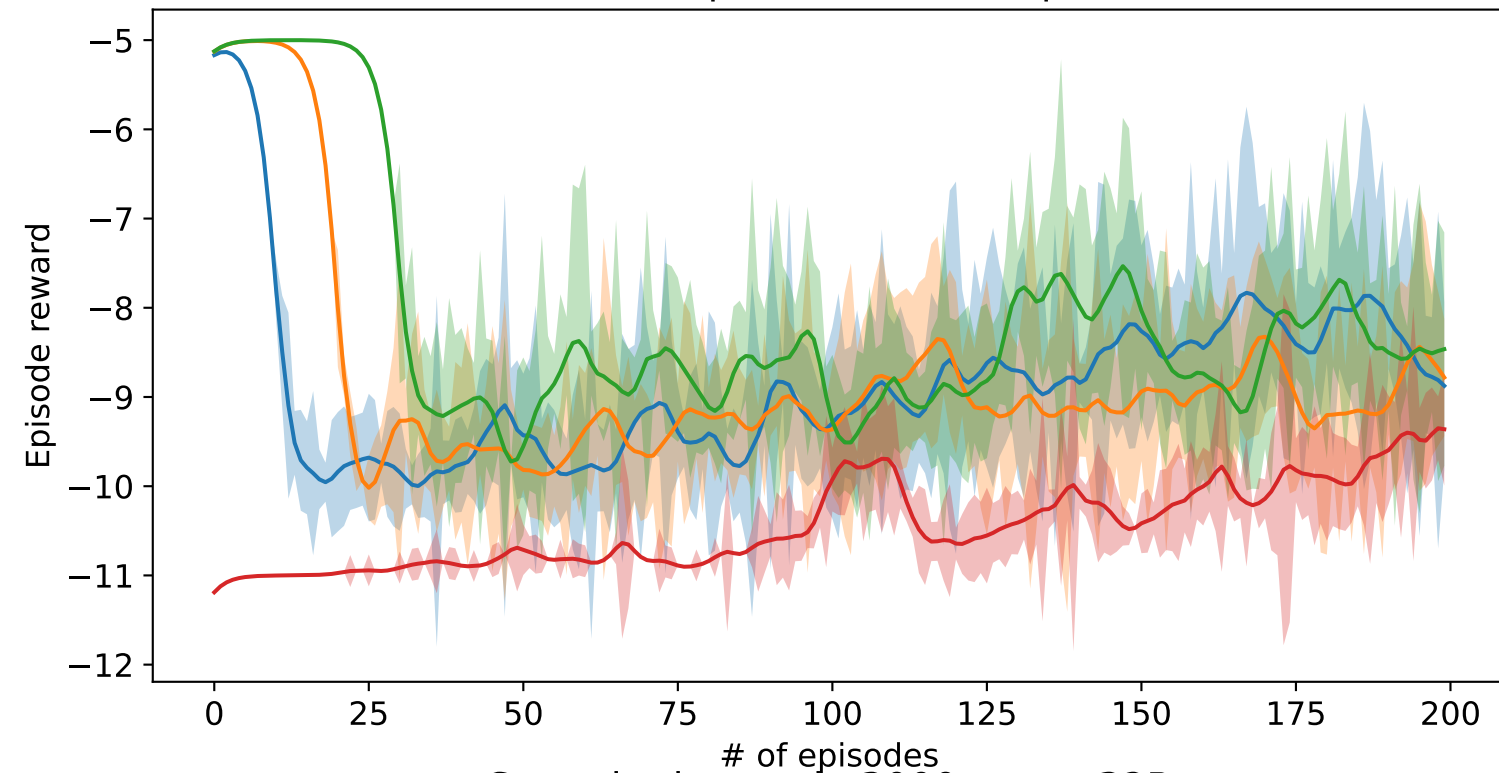
Smoothed pretrain 3000 steps, 32B
