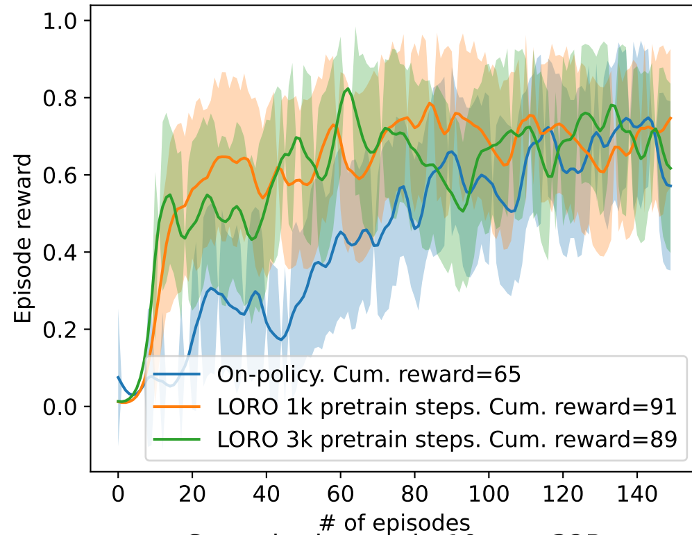
Smoothed pretrain 10 eps, 32B
