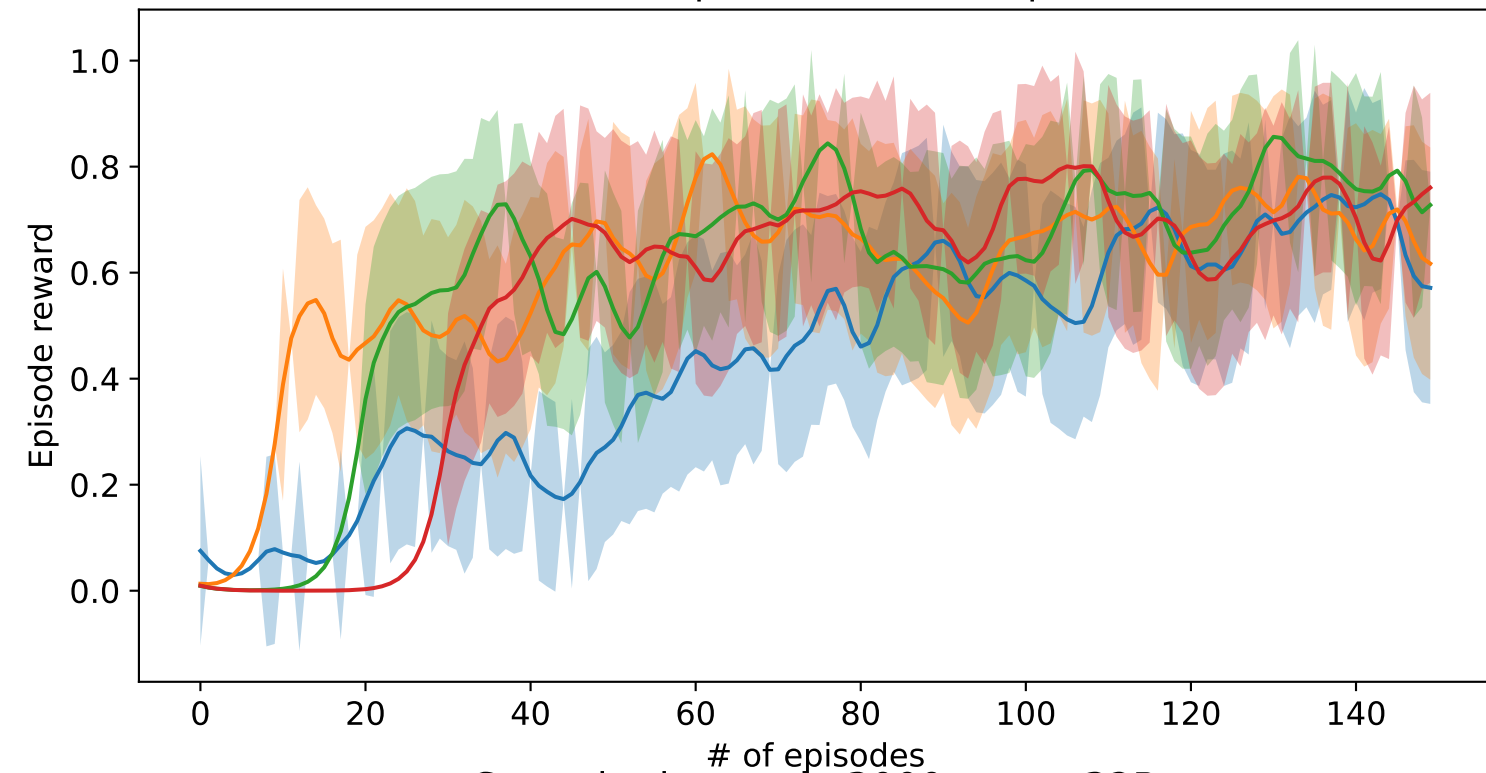
Smoothed pretrain 3000 steps, 32B
