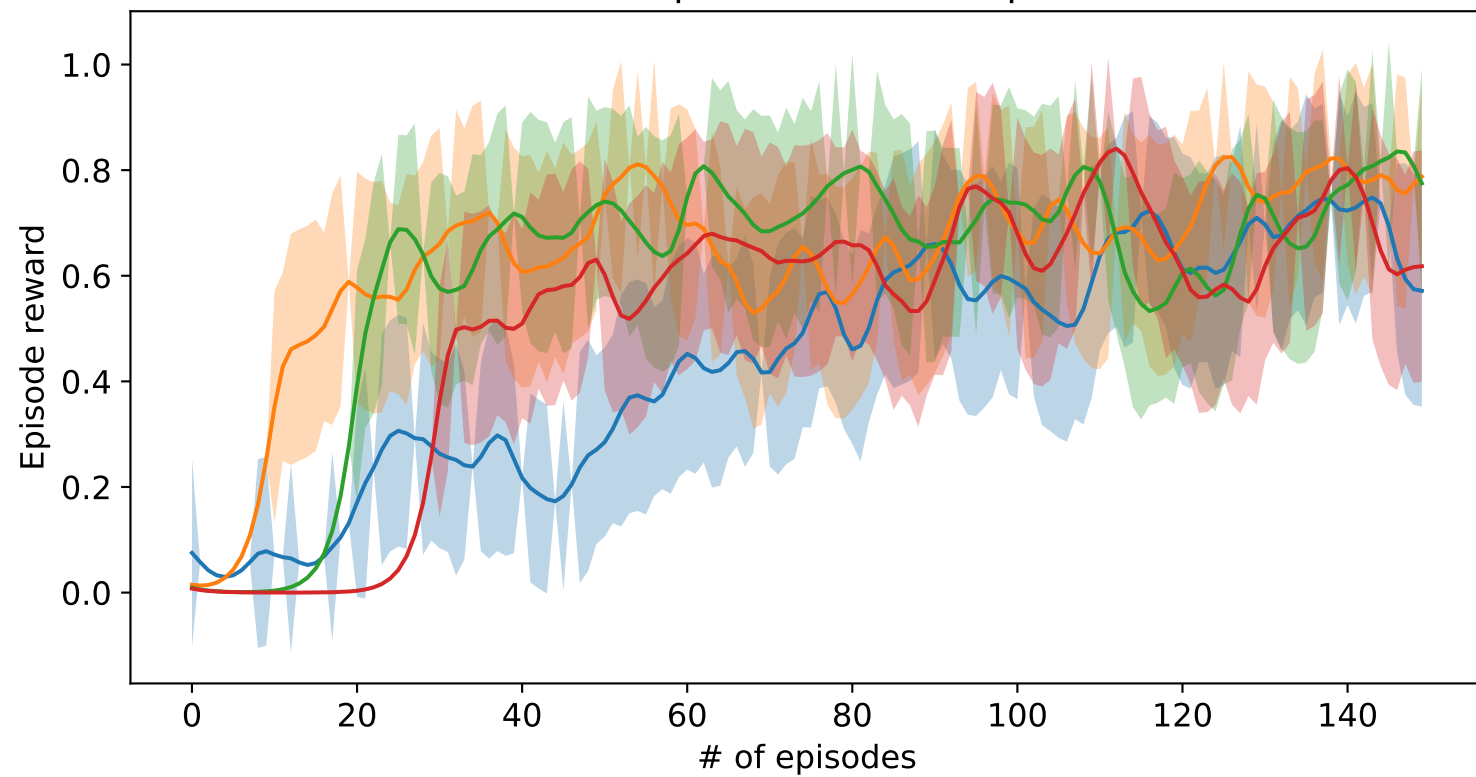
Smoothed pretrain 1000 steps, 32B
