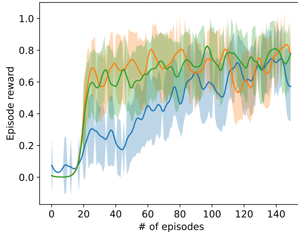
Smoothed pretrain 20 eps, 32B
