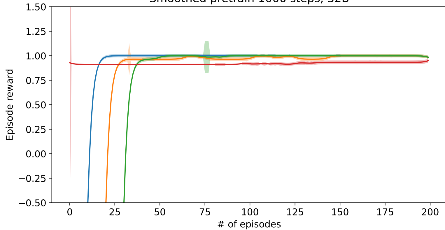
Smoothed pretrain 1000 steps, 32B
