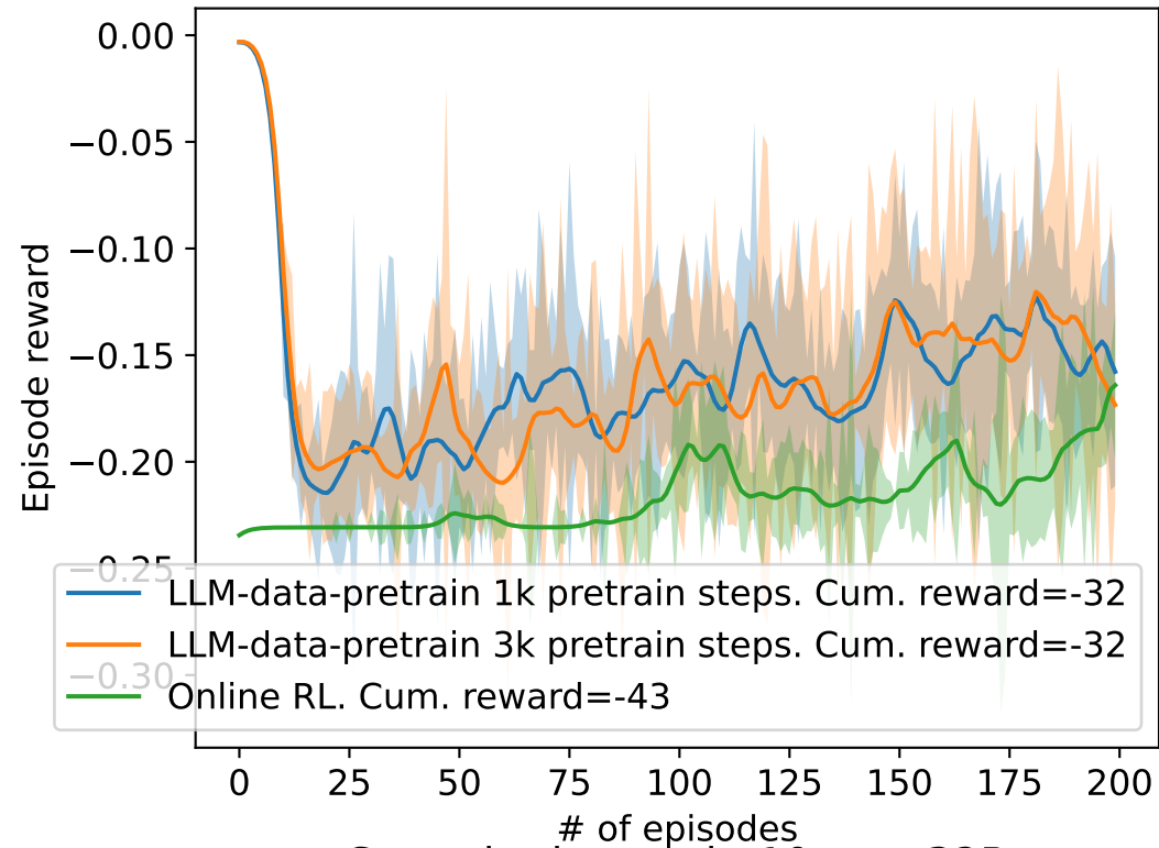
Smoothed pretrain 10 eps, 32B
