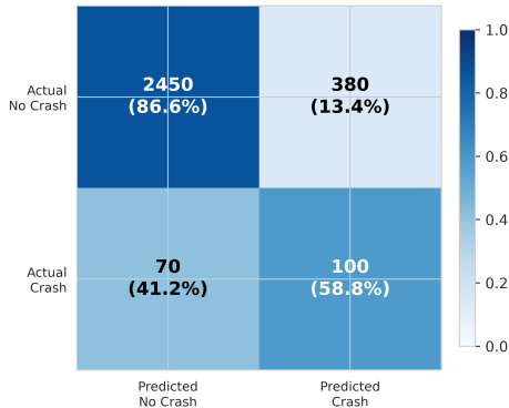
Confusion Matrix — TRR 32B (2022-23)
