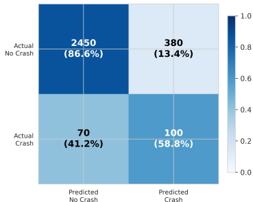
Confusion Matrix — TRR 32B (2022-23)
