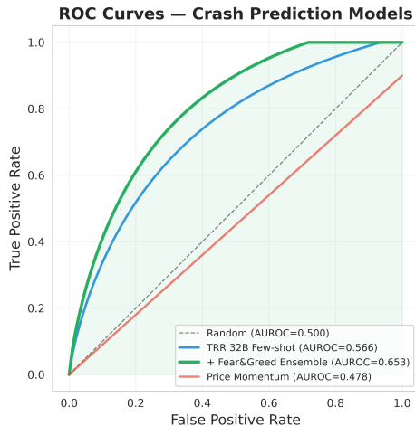
Figure 4: ROC curves for selected models. TRR ensemble dominates across all thresholds.
