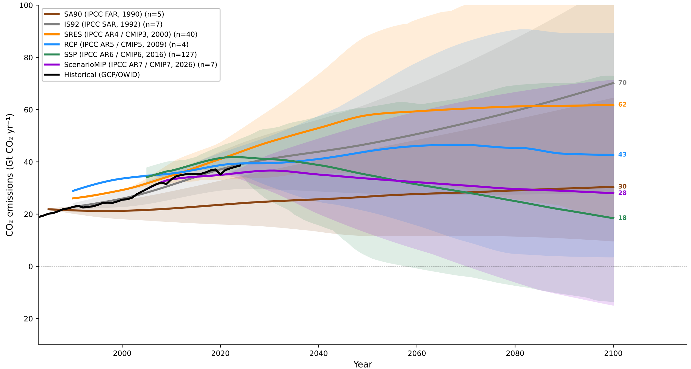
Mean CO 2 emissions trajectory per CMIP scenario generation (shading = 10th-90th percentile across all scenarios in each family)
