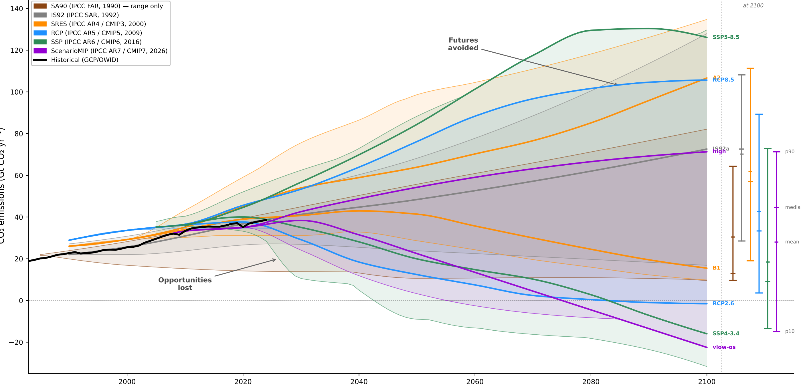
CO 2 emissions trajectories across CMIP scenario generations
