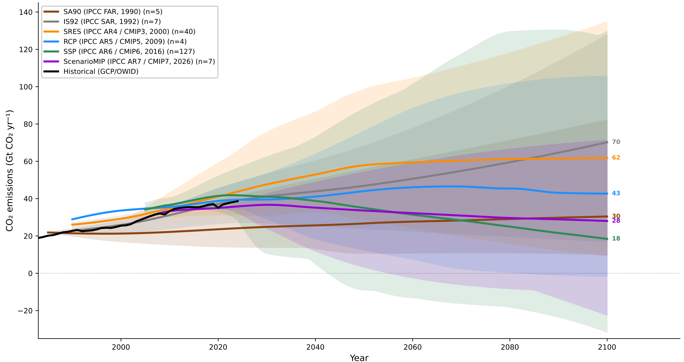
Mean CO 2 emissions trajectory per IPCC and CMIP scenario generation (shading = full scenario range across all scenarios in each family)
