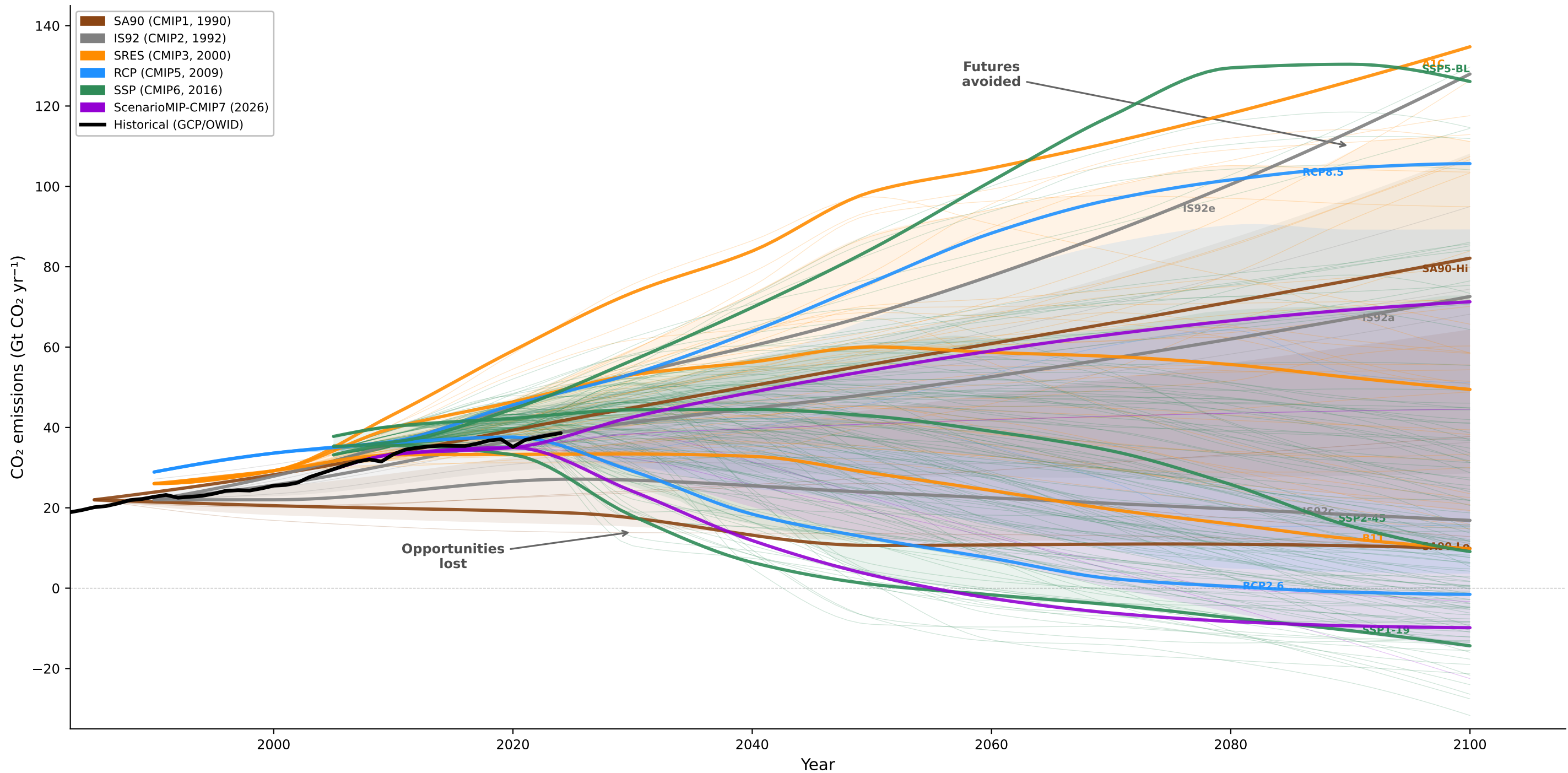
CO 2 emissions trajectories across CMIP scenario generations "Futures avoided, opportunities lost"
