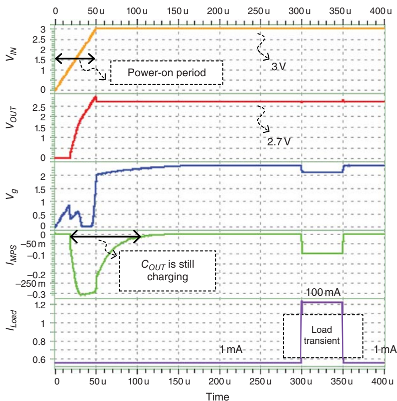
Figure 2.65 Transient response
