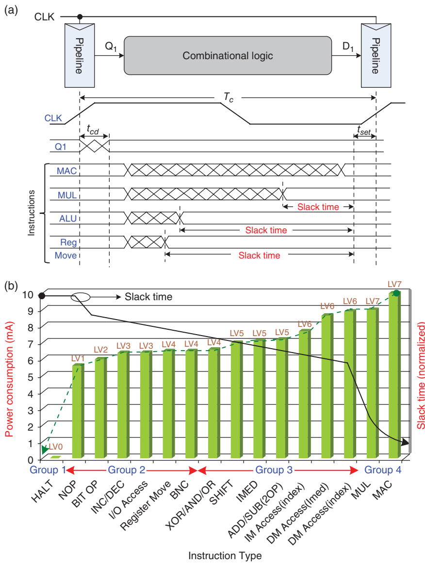
Figure 2.81 (a) Slack time in different instructions. (b) Measured slack time and power consumption in different instructions
