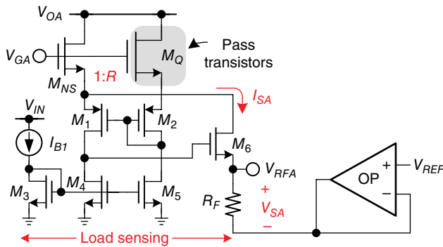
Figure 2.96 Reference adjuster in the ADVS technique
