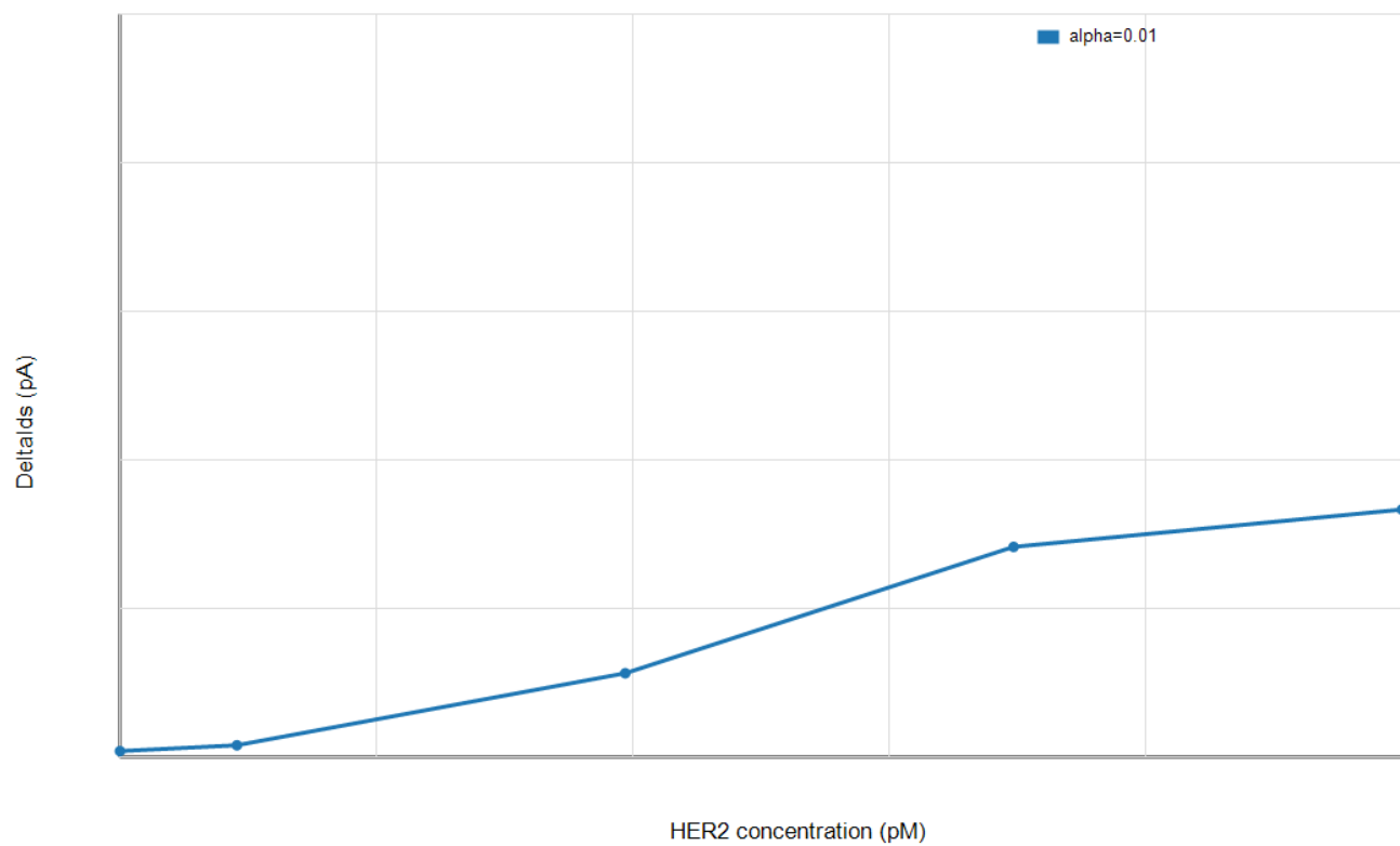
Fig. 17. GFET current response versus HER2 concentration.
