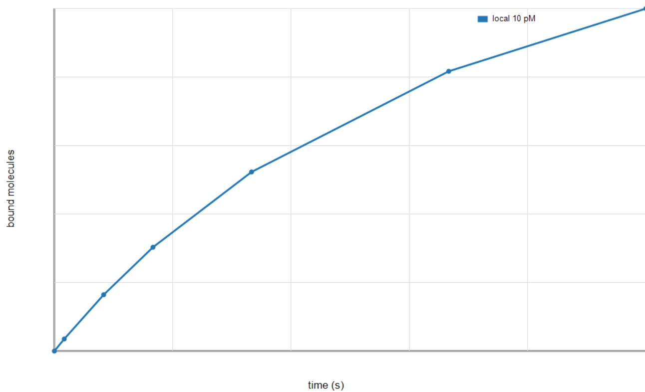
Fig. 16. Bound HER2 molecule count over time for local sensing at 10 pM.
