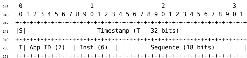
Figure 2: SKID 64-bit field layout (IETF RFC diagram convention).
