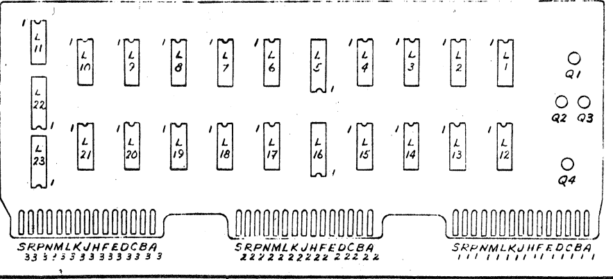
COMPONENT LAYOUT 5966
