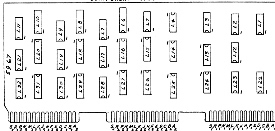
COMPONENT LAYOUT
