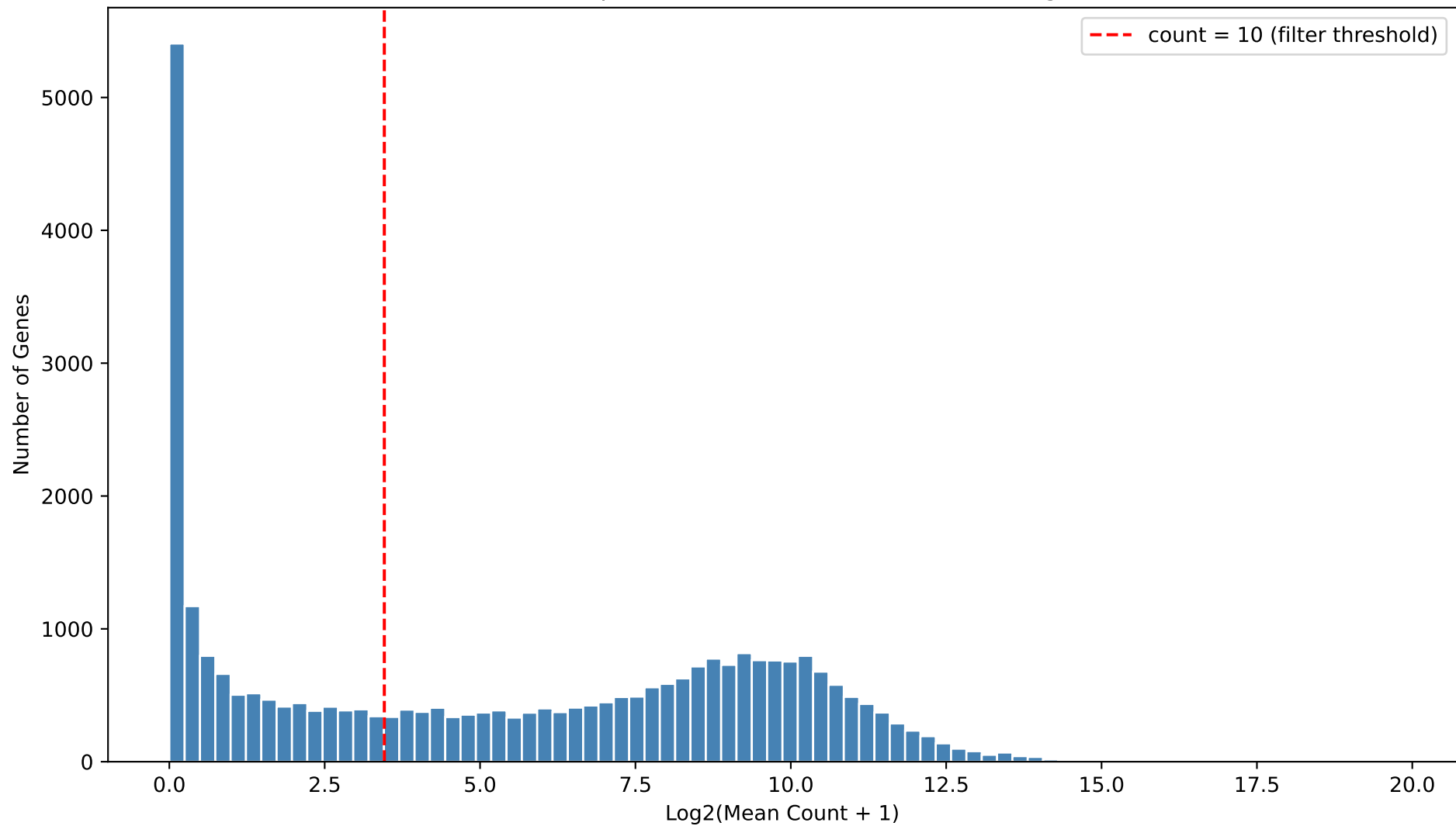
Gene Expression Distribution (before filtering)
