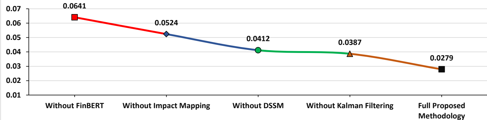
RMSE
