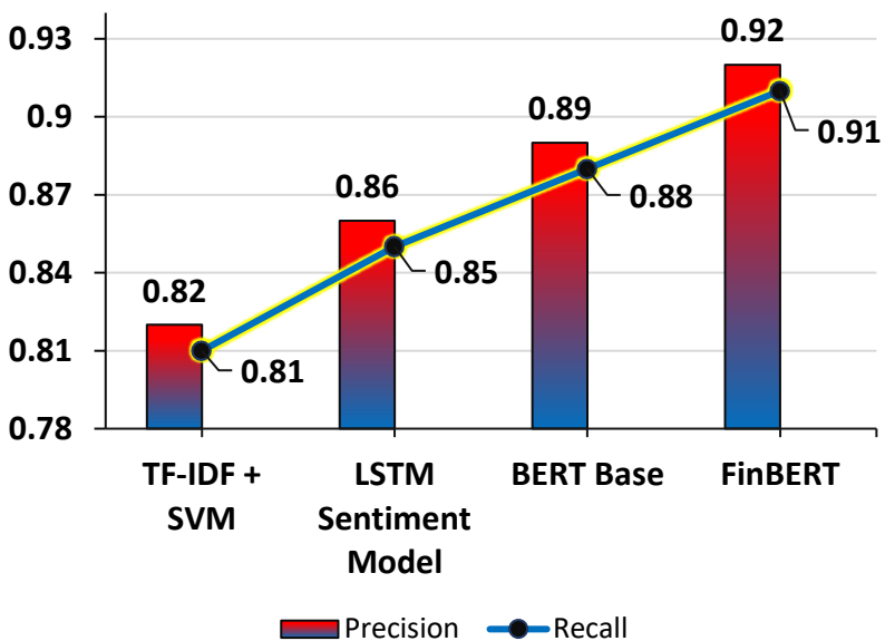
Precision and Recall
