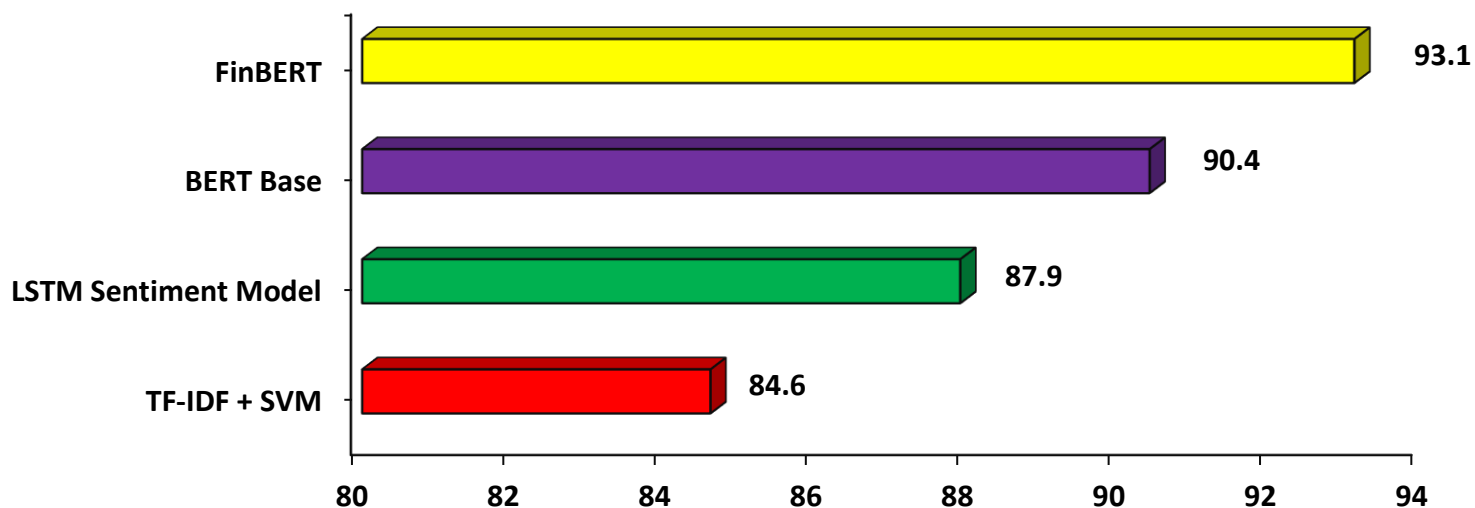
Accuracy
