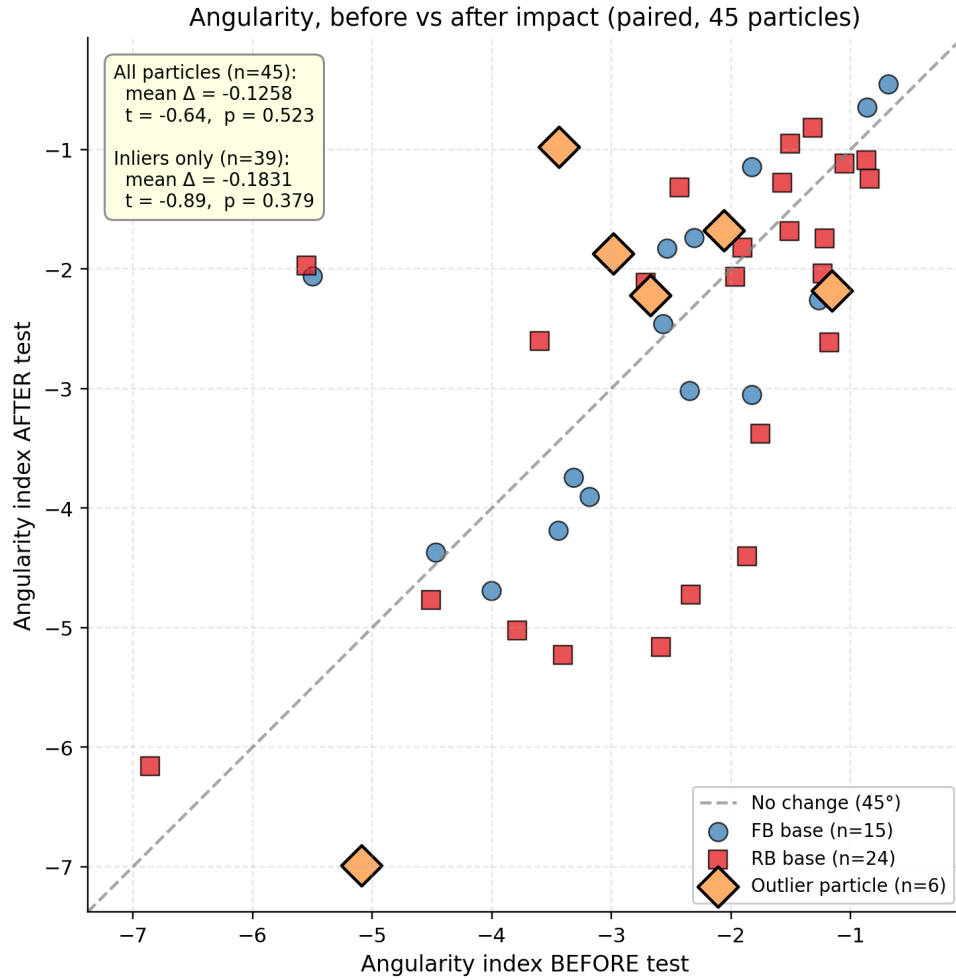
Figure 5.2. Angularity index before vs. after the impact-loading test for all 45 tracer particles. The angularity values reported here are negative scalars; less-negative (closer to zero) values indicate smoother corners.
