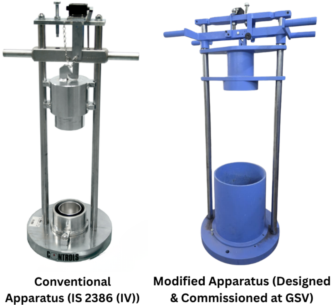
Figure 1.2. Comparison of the modified impact-testing apparatus designed and commissioned at GSV against the conventional aggregate impact value apparatus.
