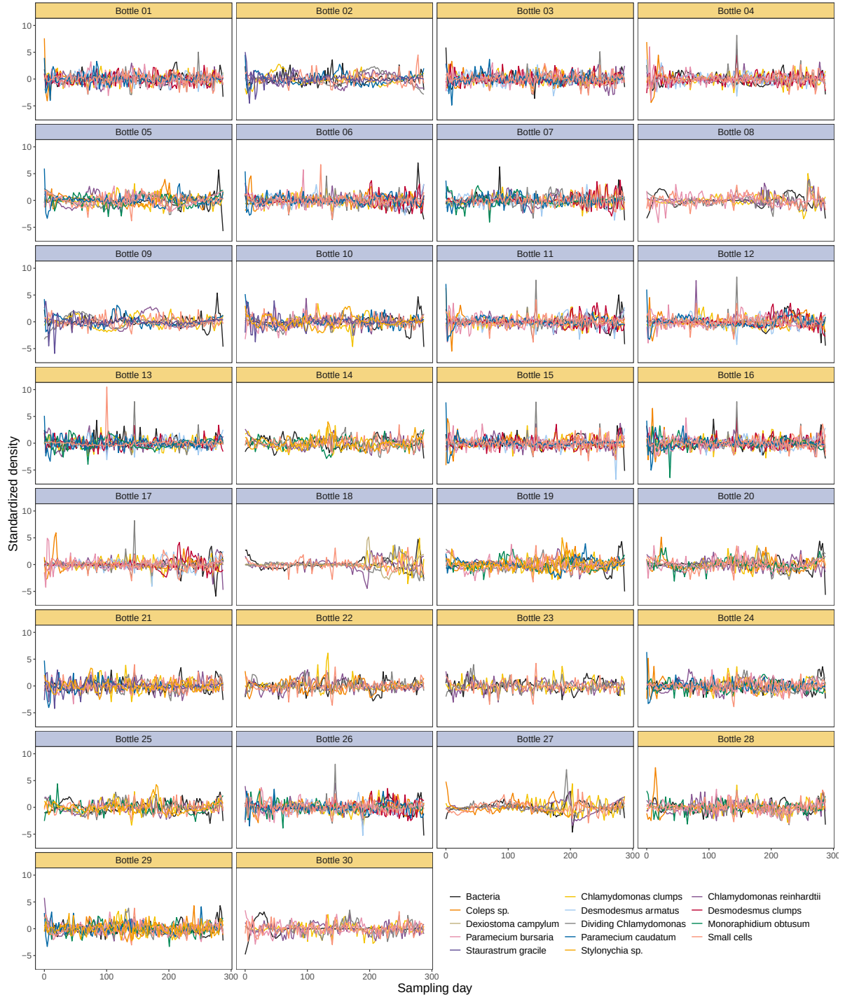
Figure 19: Time series detrending based on the segmented temporal regression. The transformed biotic density time series that were used as forecast targets, shown in the different bottles (i.e. the panels). The time series are coloured by forecast target. The background colour of the subpanel strips indicates whether the bottles were in a constant (orange) or in a decreasing (blue) light environment.
