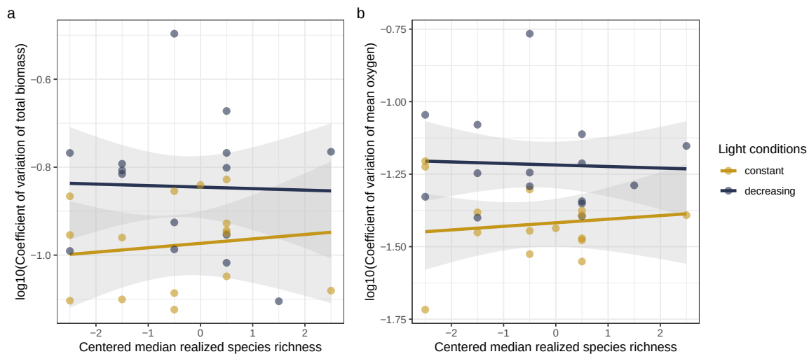
Figure 23: Coefficient of variation of (a) total community biomass, and (b) oxygen concentration. Lines display the fit of the corresponding linear mixed model, shaded areas denote the 95% confidence intervals. Incubator and composition were included as random effects in the model.
