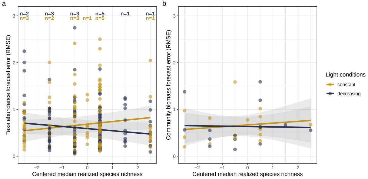
Figure 1: Effects of species richness and light on forecast error. The two treatments had interactive effects on forecast error of species abundances (a) but no effect on the forecast error of community biomass (b). Forecasts were computed with Simplex EDM, and forecast error was calculated as root mean square error (RMSE). Observed richness deviated from planned richness because not all species persisted throughout the experiment. We therefore used realized richness (i.e. the median of the observed richness values) as explanatory variable. Median richness was centered; a centered median richness of zero corresponds to a median richness of 5.5 (minimum median richness: 3; maximum median richness: 8). Lines display the fit of the linear mixed model; shaded areas denote the 95% confidence intervals. In (a), each point represents a forecasted taxon in a bottle. Taxon, bottle, and incubator were included as random intercepts in the model. Inserts at the top indicate the number of bottles for the respective richness level (yellow: constant light, blue: decreasing light). In (b), bottle and incubator were included as random intercepts in the model.
