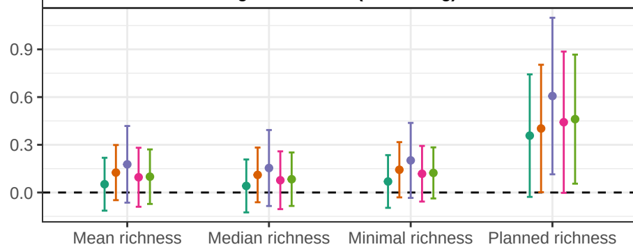
Interaction: light conditions and species richness
