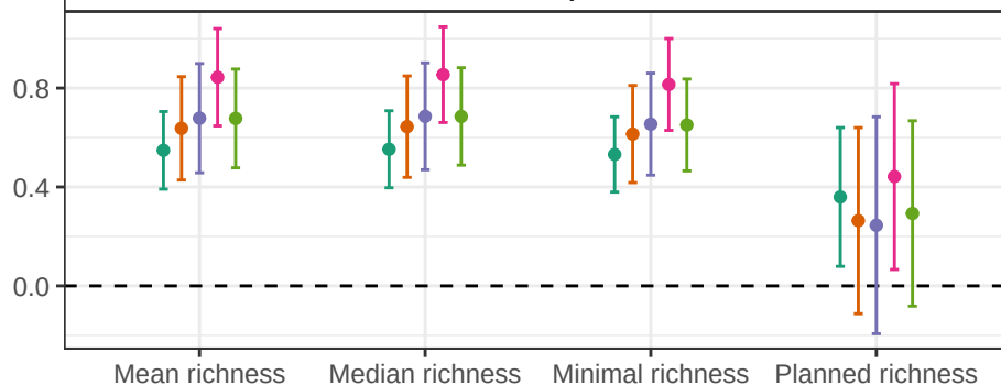
Species richness
