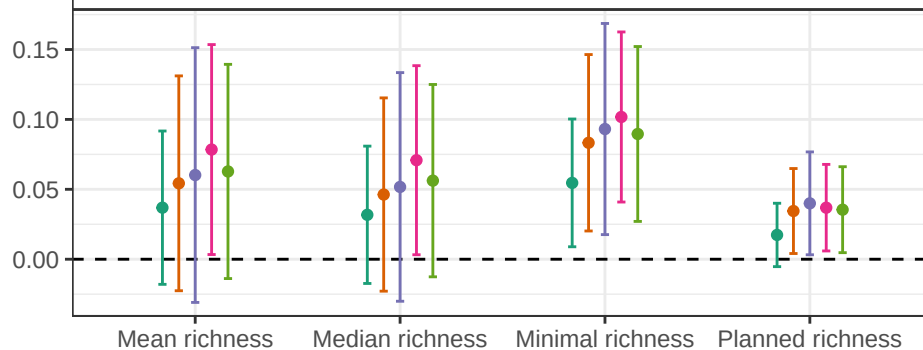
Species richness
