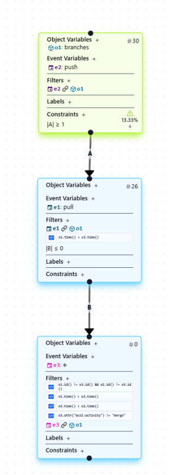
Figure 2: OCPQ query for C1 (three nested nodes) and result: 4 of 30 pushes violate C1 (86.67% compliance).
