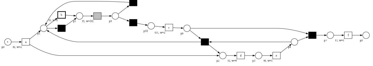
Figure 1: The GSLPN from the assignment (p.6), redrawn from the encoding used by q3_gslpn.py ( poetry run q3 ). Layout differs from the original figure (auto-generated left-to-right), but the places, transitions, weights and arcs are identical. Legend: plain box = timed, thick-bordered box = immediate (visible), grey box = \tau and timed, black box = \tau and immediate.
