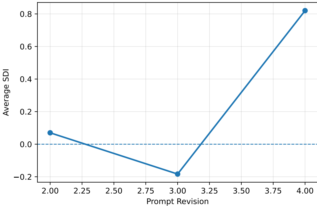
Security Drift Index Across Prompt Revisions
