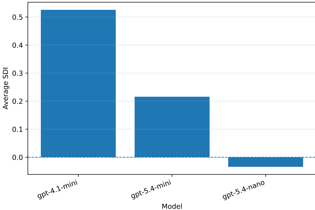
Average Security Drift by Language Model
