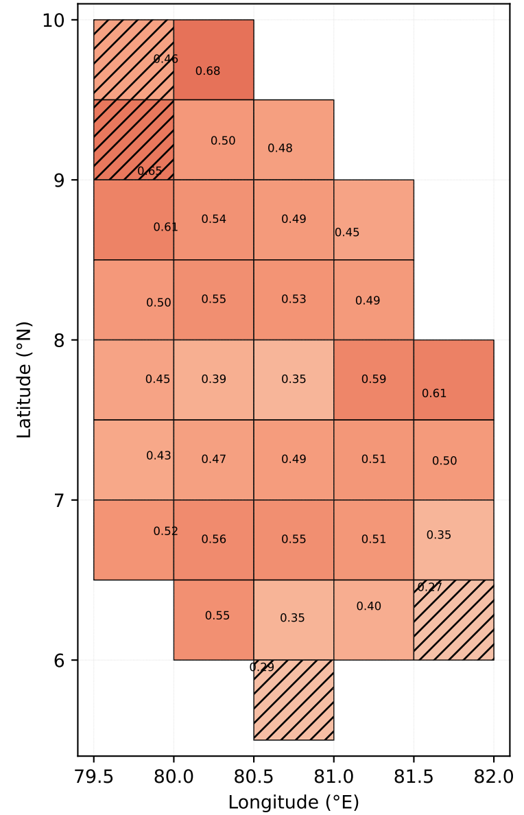
Same-month seasonal correlation between precipitation and soil moisture
