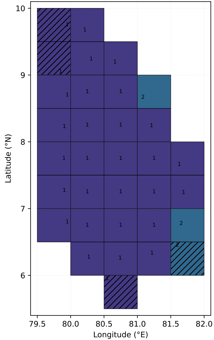
Best antecedent precipitation lag for monthly soil moisture
