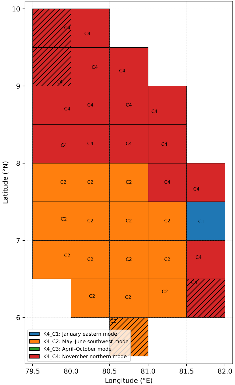
Dominant annual precipitation component
